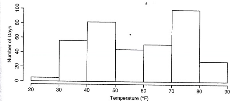
Figure 14.2. Histogram of 2010 Albuquerque temperatures
