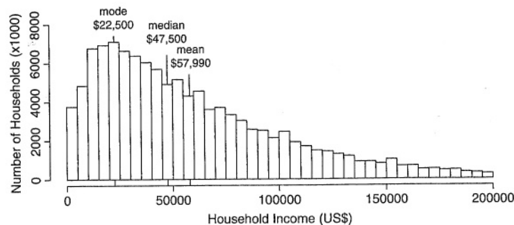
Figure 14.6. Histogram of 2009 household income, with central tendencies labeled
