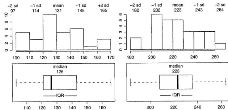
Figure 14.7. Dispersion of Peterson and Barney F0 for men and women
