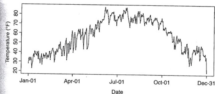
Figure 14.8. Plot of 2010 Albuquerque temperatures by date
