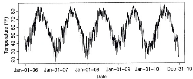
Figure 14.9. Plot of 2006–2010 Albuquerque temperatures by date
