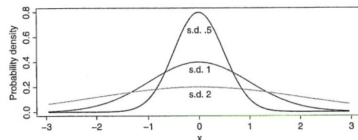
Figure 14.5. Three normal distributions: mean = 0, standard deviations = {0.5, 1, 2}
