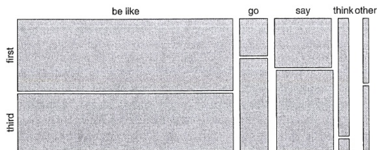
Figure 14.15. Mosaic plot of York quotative variants by grammatical person
